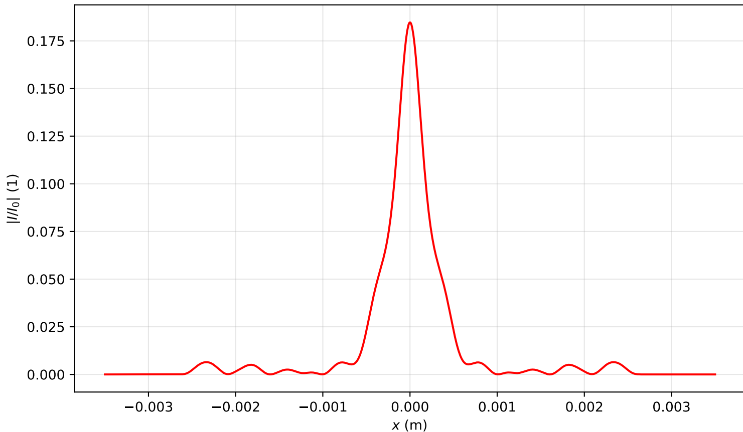
Intensity profile I(x, y = 0, z = 3.184)/I_0 , Pin=8.0Pcr, artificial time
